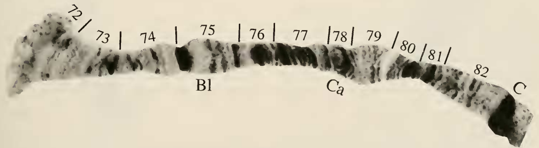
Fig. 7. Chromosome arm IIS of Simulium parnassum , with landmarks of Rothfels et al. (1978). C = centromere region. Section numbers are those of both S. parnassum standard banding sequence and Simulium subgeneric standard of Rothfels et al. (1978). Male from South Carolina, Pickens Co., Oil Camp Creek, 8 May 1998. Bl = blister, Ca = capsule.
